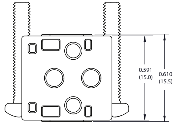
2-Way 15 mm High Flow Series BP15-2HV
