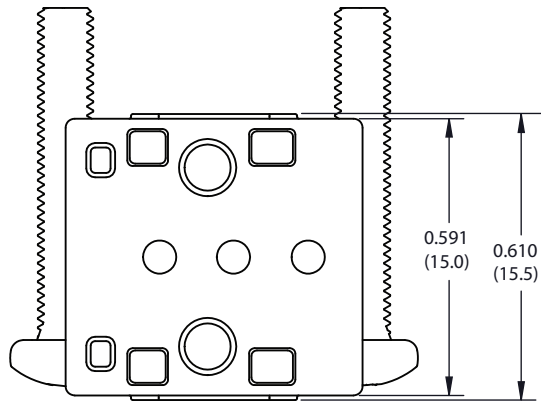
2-Way & 3-Way 15 mm Standard Series BP15-3SV
